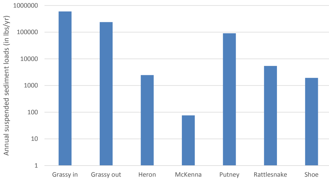
Figure 3: Annual suspended sediment loads (in lbs/yr) for Barbee stream sites. Note that scale on vertical axis is logarithmic to show smaller and larger loads on same figure.
