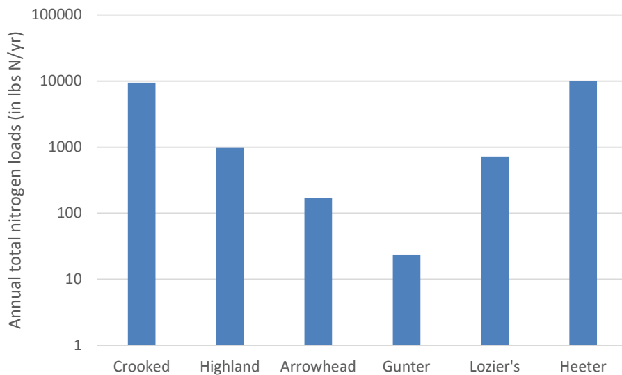
Figure 8: Annual total nitrogen loads (in lbs N/yr) for Chapman stream sites. Note that scale on vertical axis is logarithmic to show smaller and larger loads on same figure.
