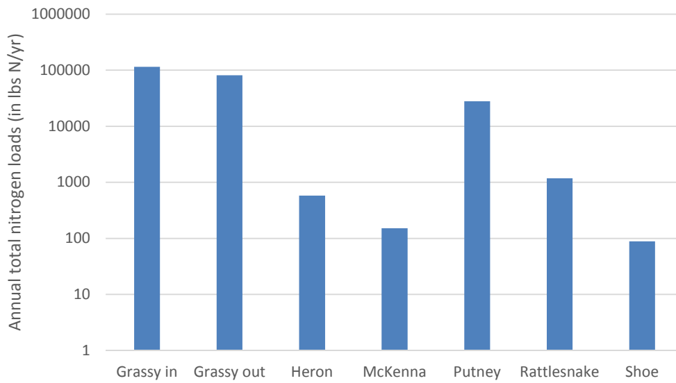
Figure 5: Annual total nitrogen loads (in lbs N/yr) for Barbee stream sites. Note that scale on vertical axis is logarithmic to show smaller and larger loads on same figure.
