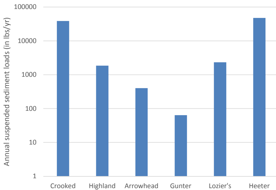
Figure 6: Annual suspended sediment loads (in lbs/yr) for Chapman stream sites. Note that scale on vertical axis is logarithmic to show smaller and larger loads on same figure.
