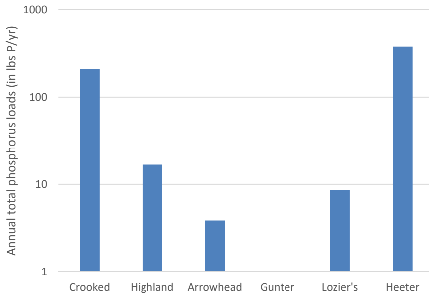
Figure 7: Annual total phosphorus loads (in lbs P/yr) for Chapman stream sites. Note that scale on vertical axis is logarithmic to show smaller and larger loads on same figure.
