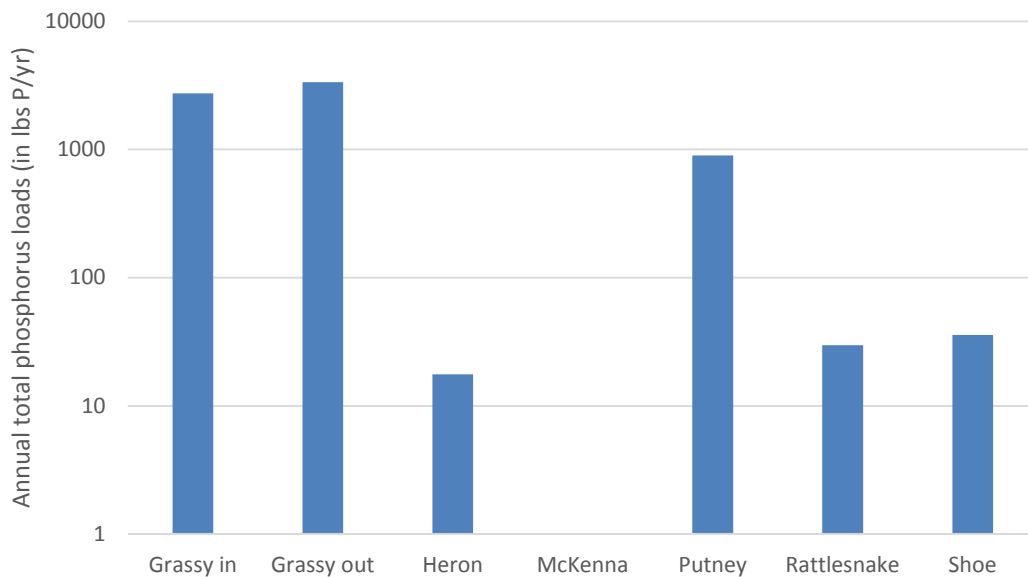
Figure 4: Annual total phosphorus loads (in lbs P/yr) for Barbee stream sites. Note that scale on vertical axis is logarithmic to show smaller and larger loads on same figure.
